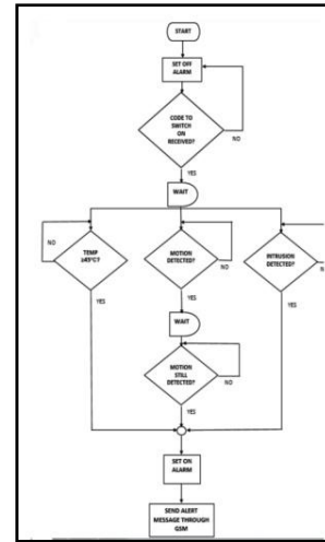
Fig.4.1: Working Algorithm
